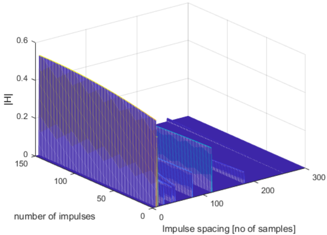
Channel Impulse Response for LTE fading channel Rx Antenna1
